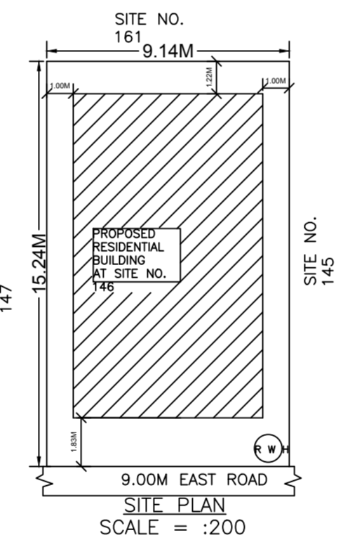
SITE PLAN SCALE = :200
