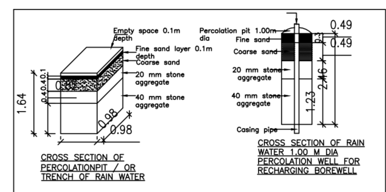
CROSS SECTION OF PERCOLATION PIT / OR TRENCH OF RAIN WATER
