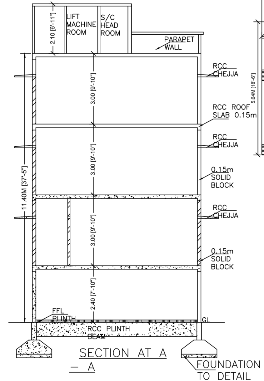
SECTION AT A - A FOUNDATION TO DETAIL
